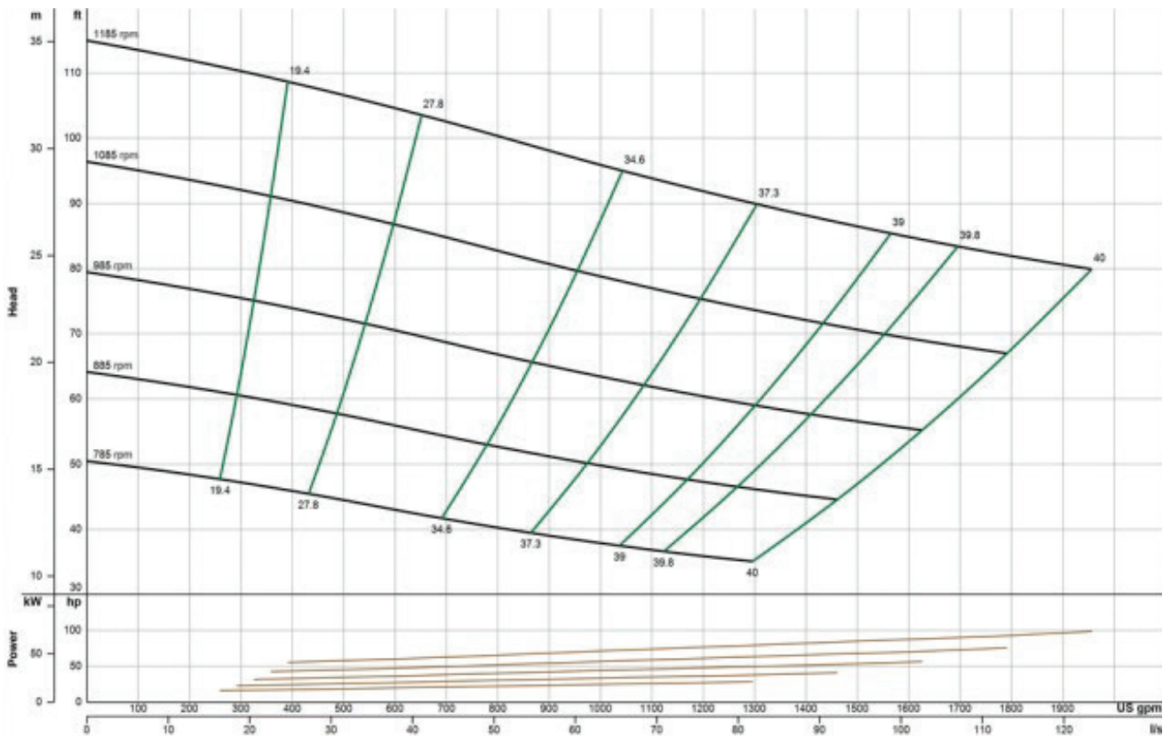
EDDY Pump - Self-Priming Pump 6-inches 173-HP - Pump Curvez
