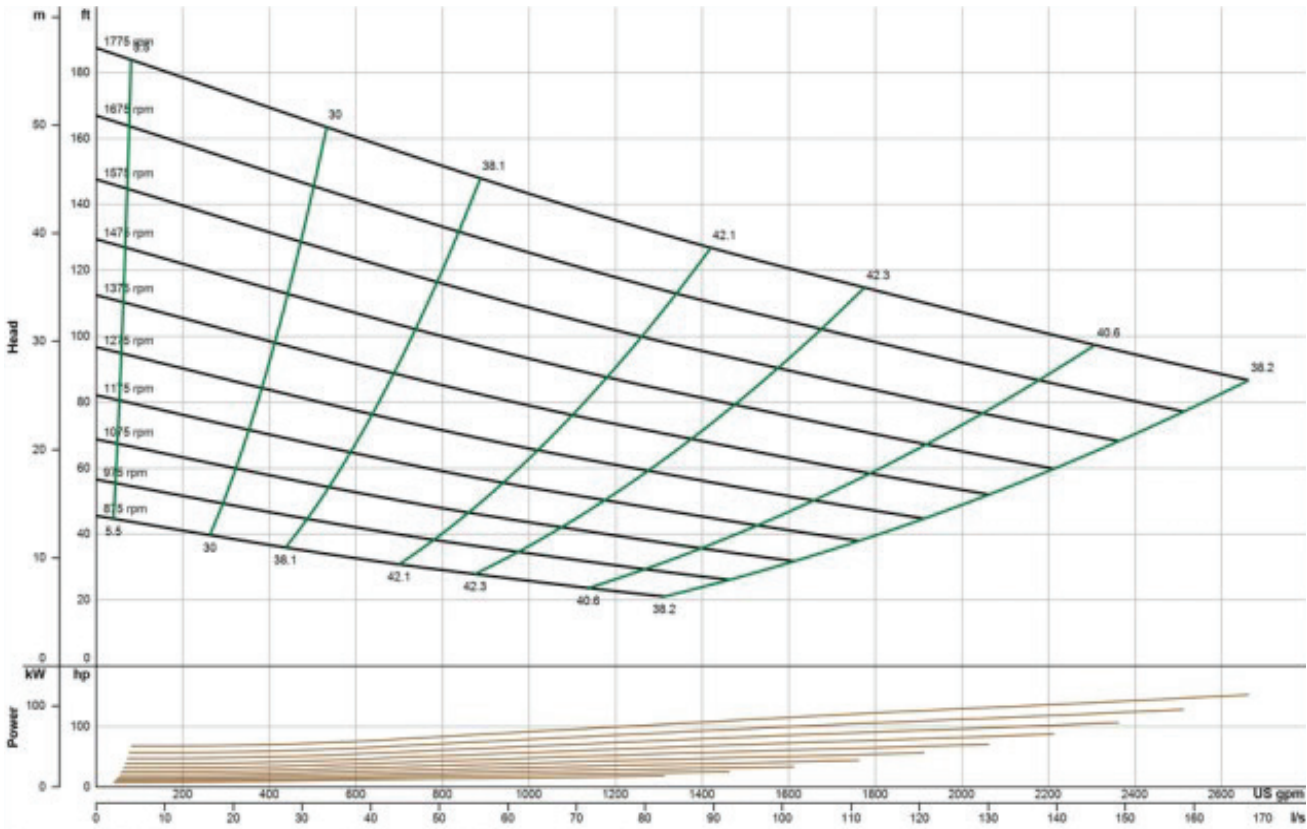
EDDY Pump - Self-Priming Pump 4-inches 43-HP - Pump Curve
