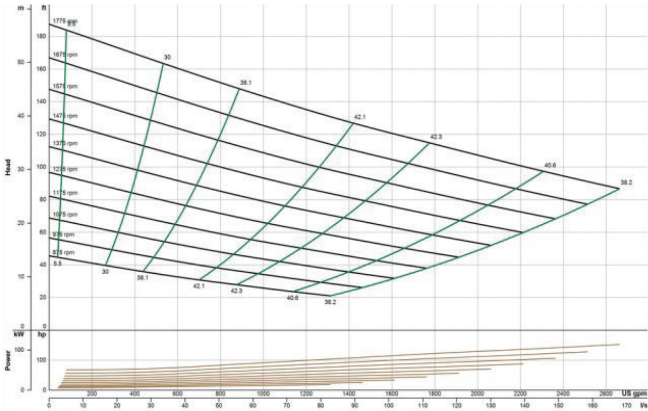
EDDY Pump - Self-Priming Pump 4-inch 115-HP - Pump Curve
