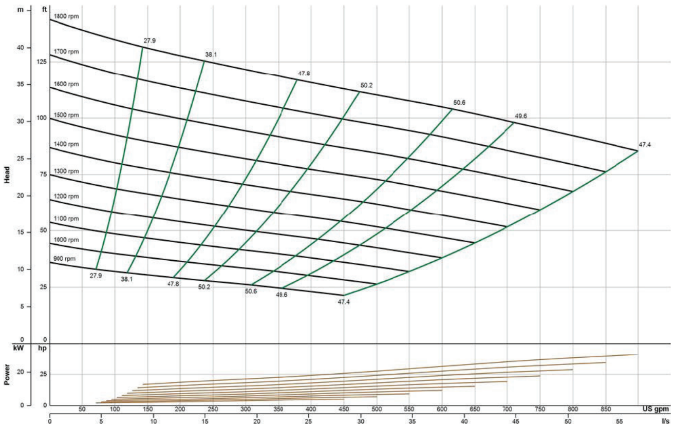
EDDY Pump - Self-Priming Pump 3-inch 43-HP - Pump Curve
