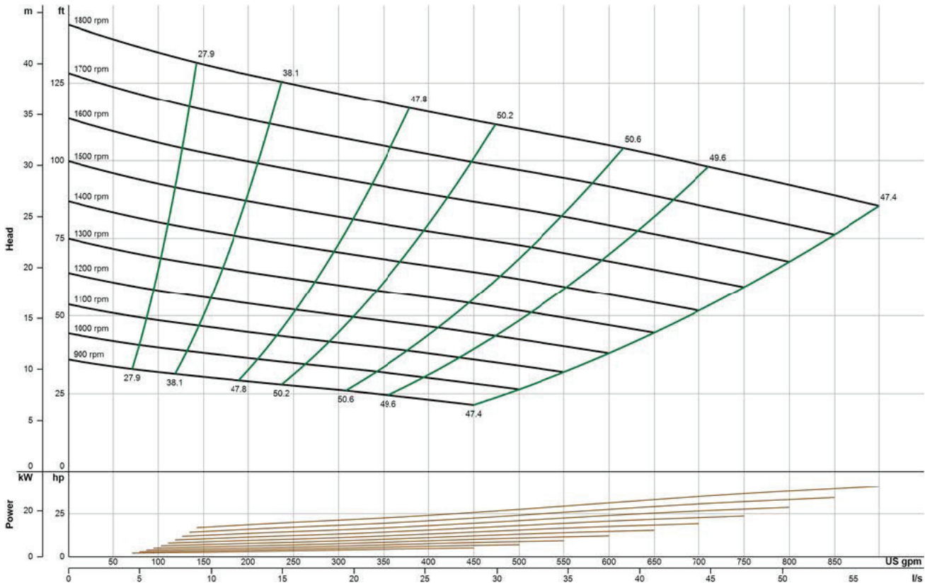
EDDY Pump - Self-Priming Pump 3-inches 43-HP - Pump Curve
