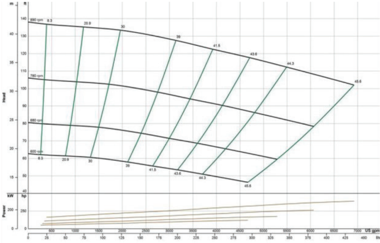
EDDY Pump - Self-Priming Pump 12-inches 700-HP - Pump Curve
