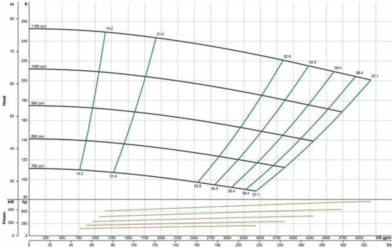
EDDY Pump - Self-Priming Pump 10-inches 550-HP - Pump Curve
