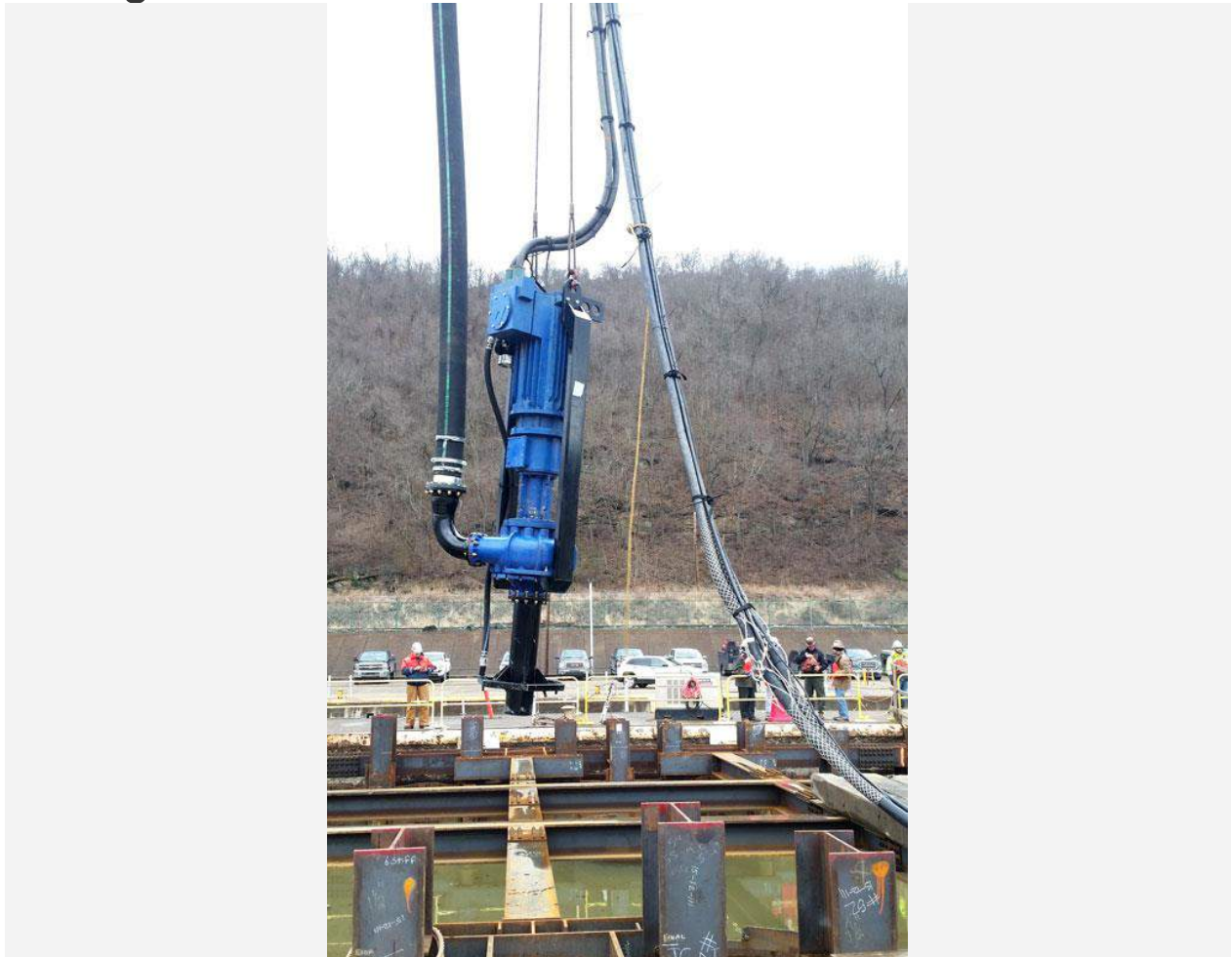
2017 Project – Canal Locking System Project. The 8-inch cable hanging dredge pump was used to remove sand for this expansion project.
