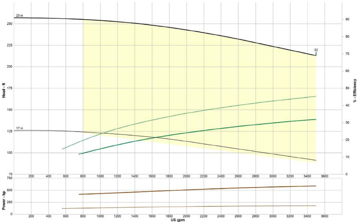
EDDY Pump - 8 Inch JPH 8000 Cable Deployed Pump - Pump Curve
