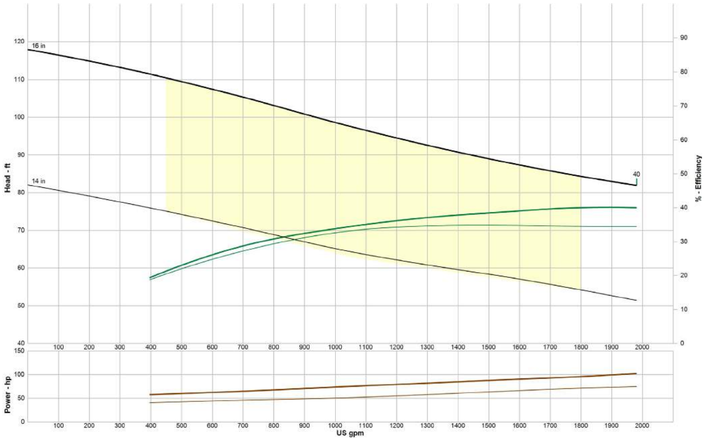
EDDY Pump - 6 Inch JPH 6000 Cable Deployed Pump - Pump Curve - Pump Curve
