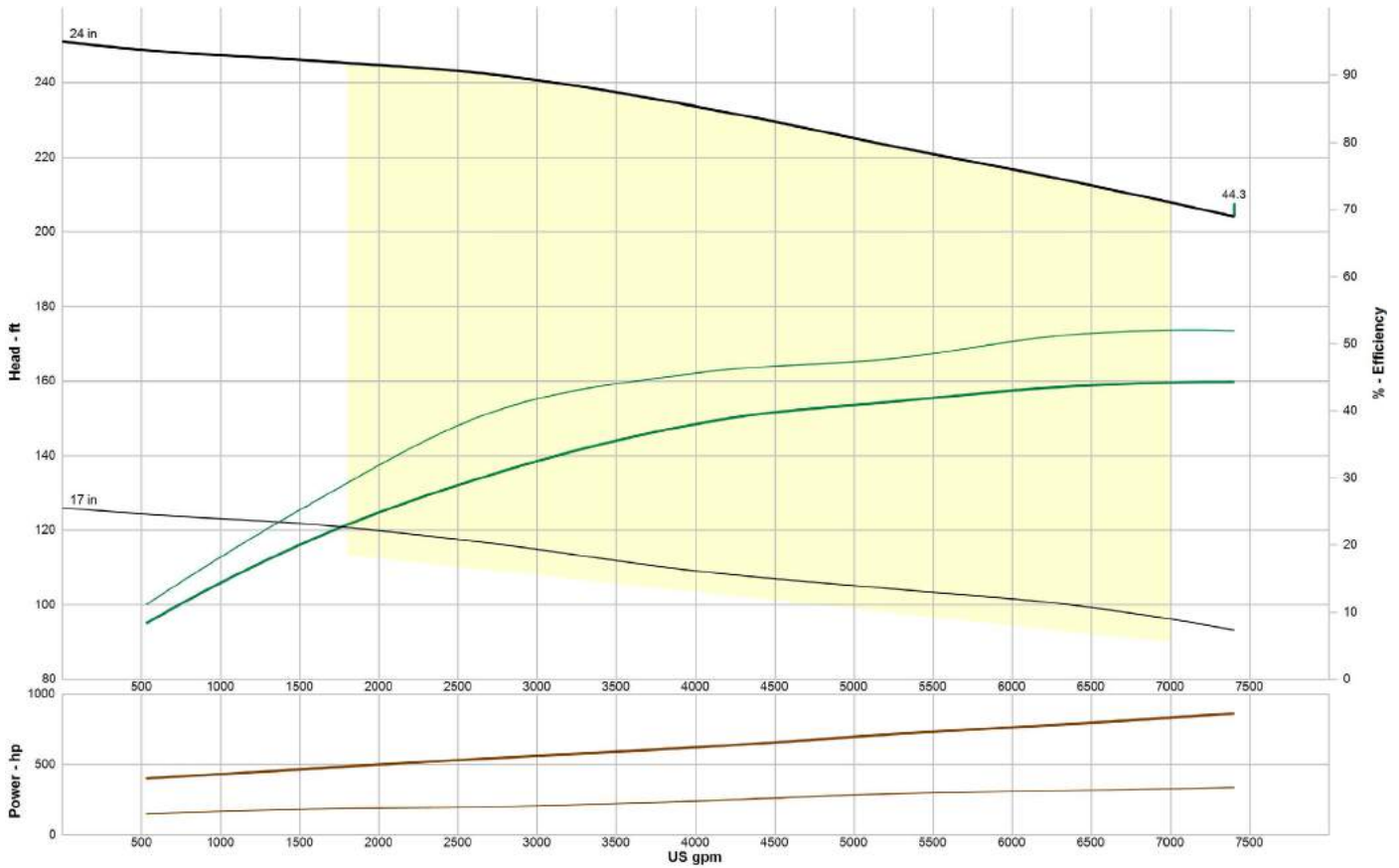
EDDY Pump - 12 Inch JPH 12000 Cable Deployed Pump - Pump Curve
