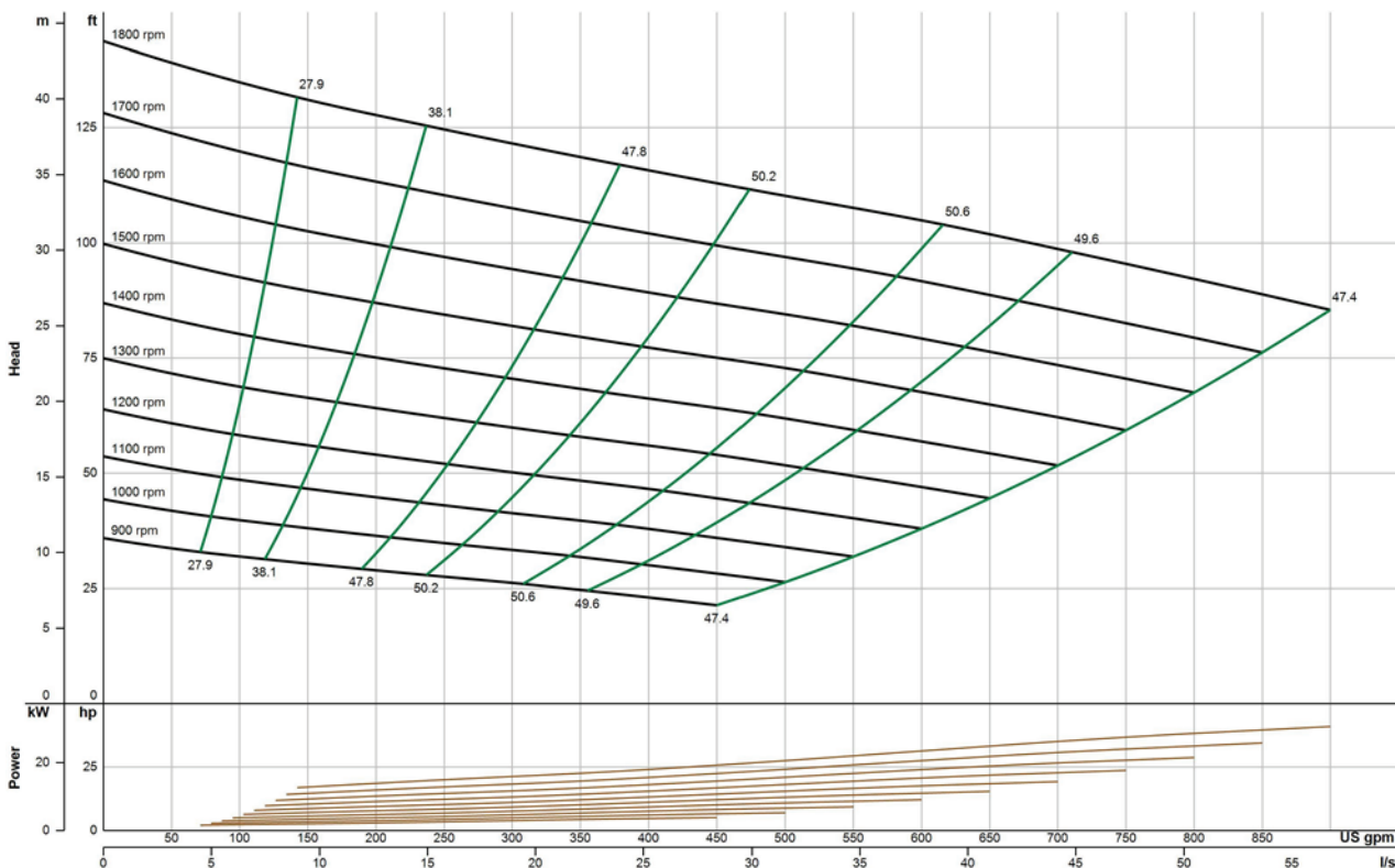
EDDY Pump - 3 Inch HD 3000 Heavy Duty Slurry Pump - Pump Curve
