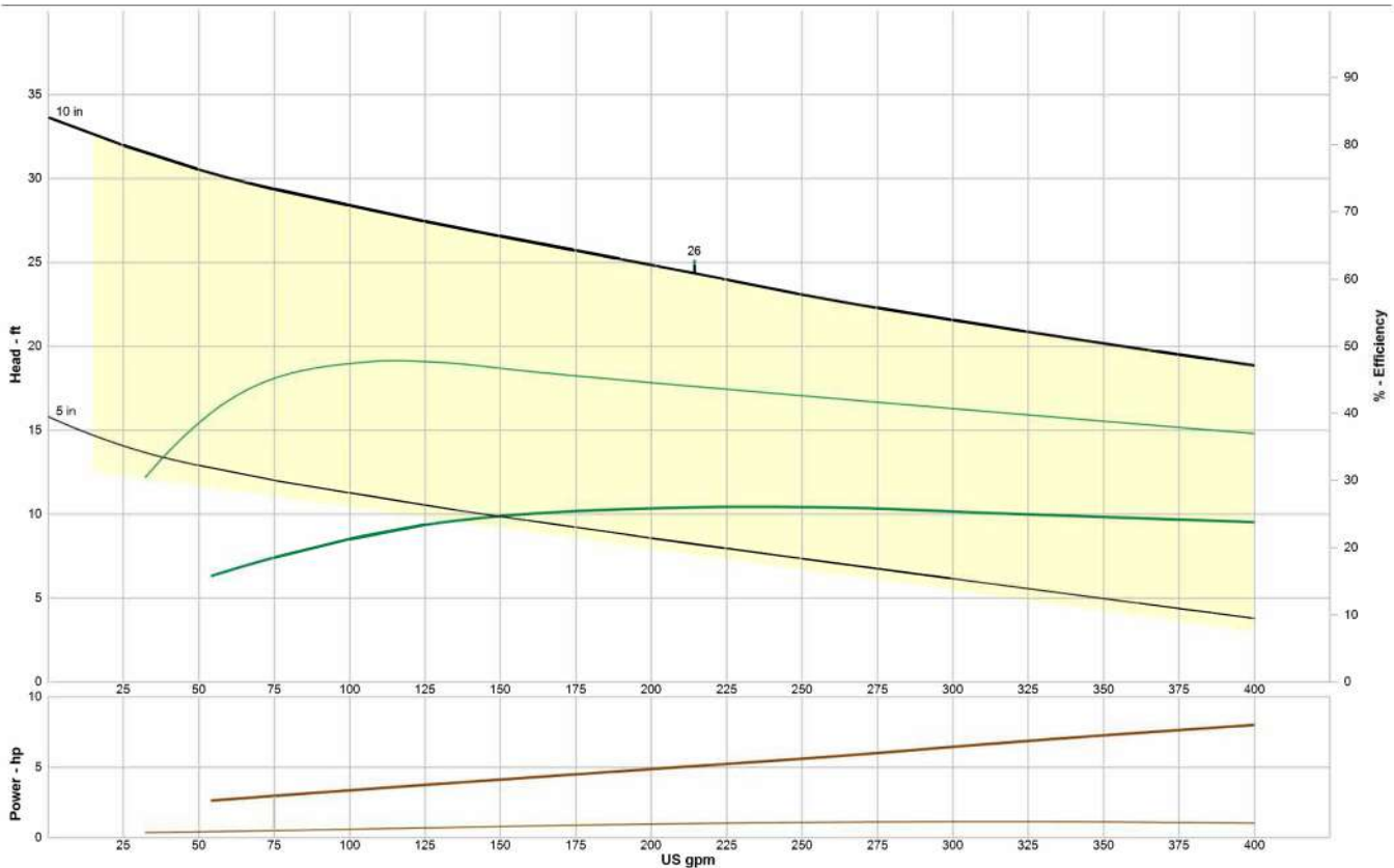
EDDY Pump - 2 Inch C 2300 Commercial Slurry Pump - Pump Curve
