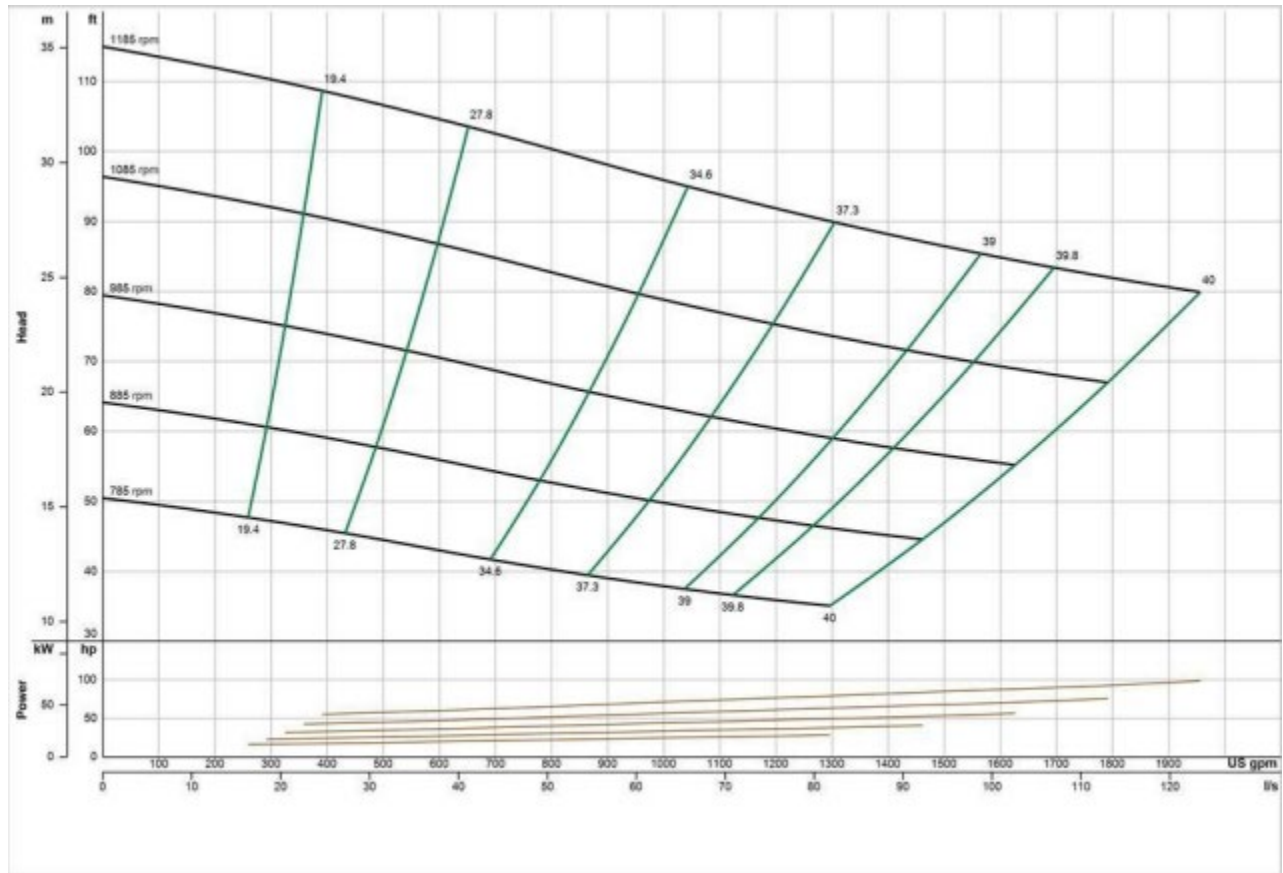
EDDY Pump - 6 Inch 6000 Heavy Duty Slurry Pump - Pump Curve
