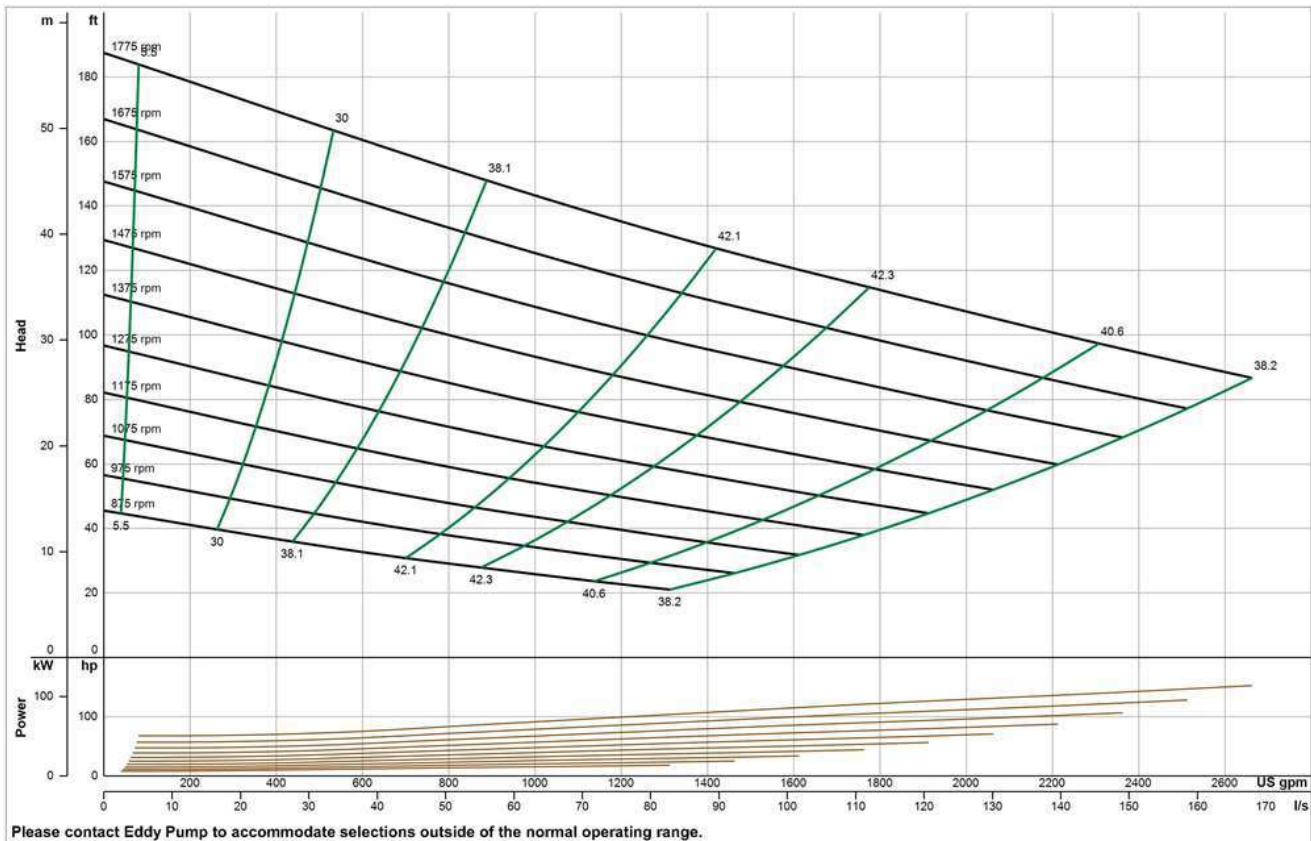
EDDY Pump – HD4K Hydraulic Diver Operated - Pump Curve
