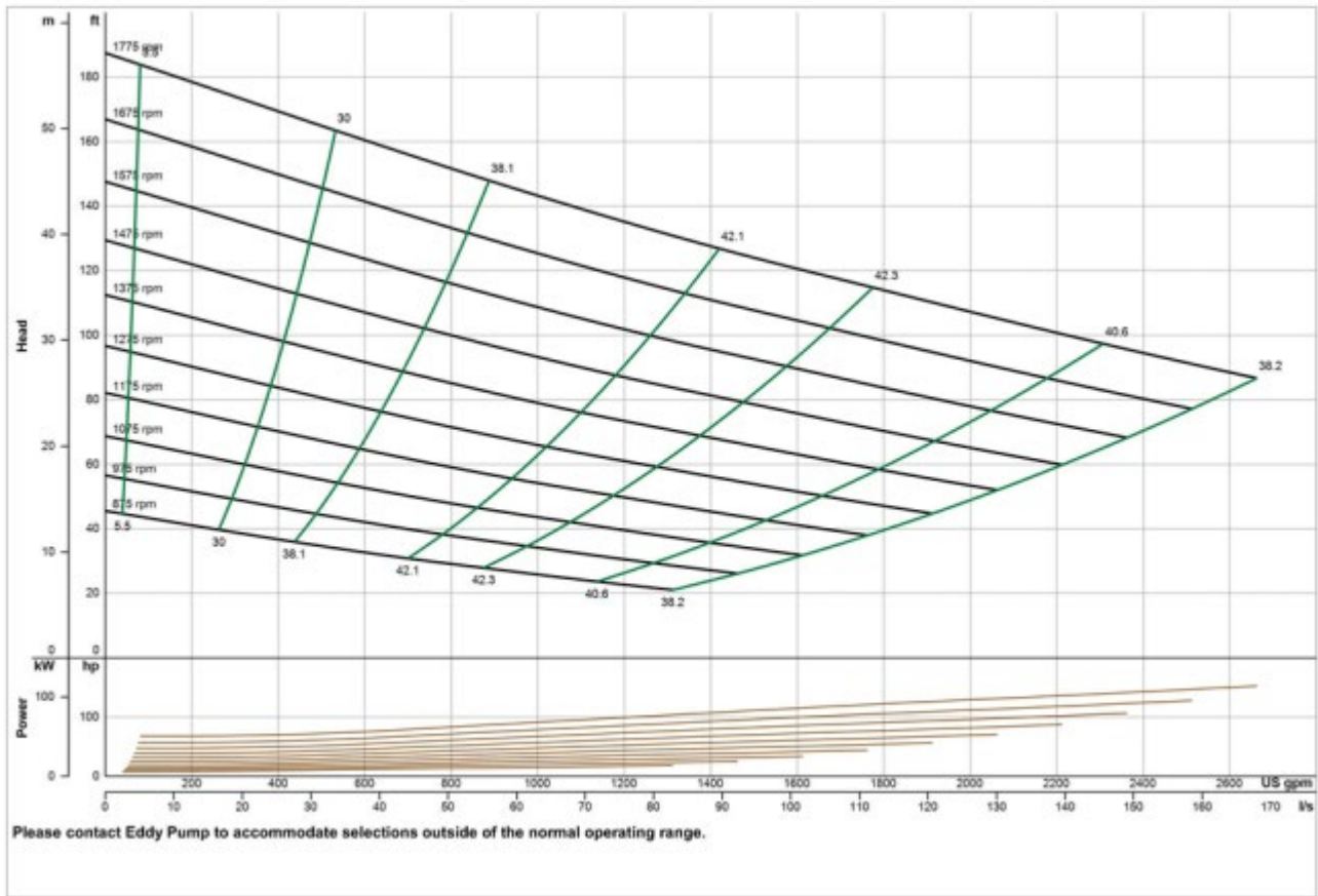
EDDY Pump - 4 Inch HD 4000 Heavy Duty Slurry Pump - Pump Curve
