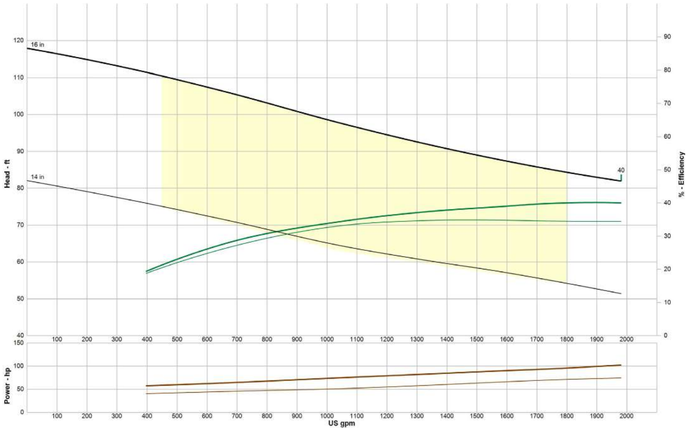
EDDY Pump - 6 Inch EXH 6000 Hydraulic Excavator Attachment - Pump Curve
